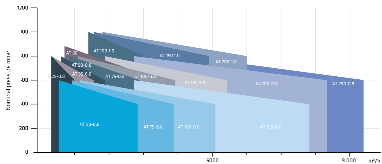
Pressure and volume flow ranges for Generation 5 plus
