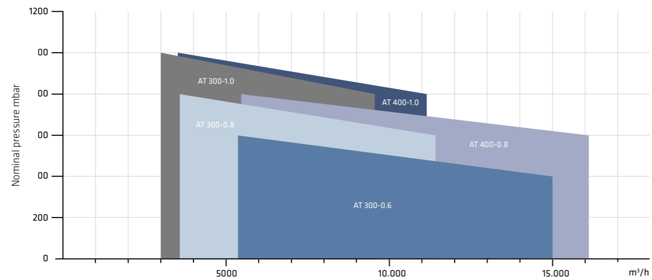
Pressure and volume flow ranges for Generation 5
